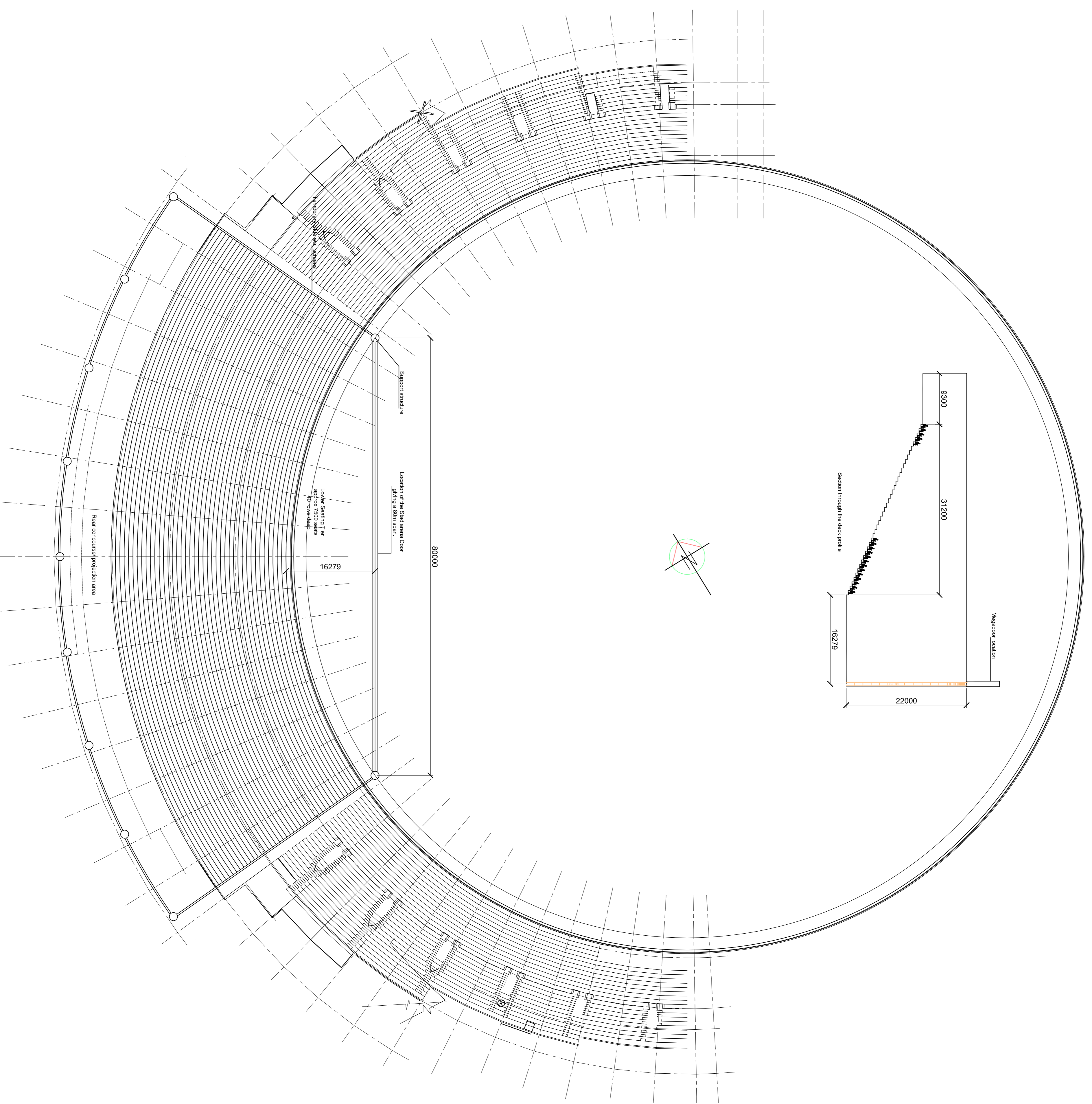
Deck Plan scale 1:400
